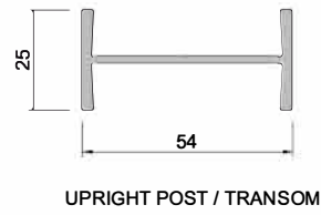
UPRIGHT POST / TRANSOM
