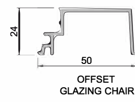
OFFSET/DOUBLE GLAZING BEAD
